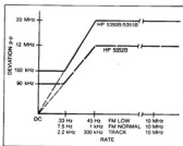
Graph 2. FM Rate Tolerance
