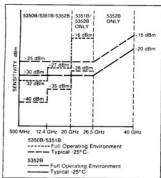
Graph 1. Sensitivity
